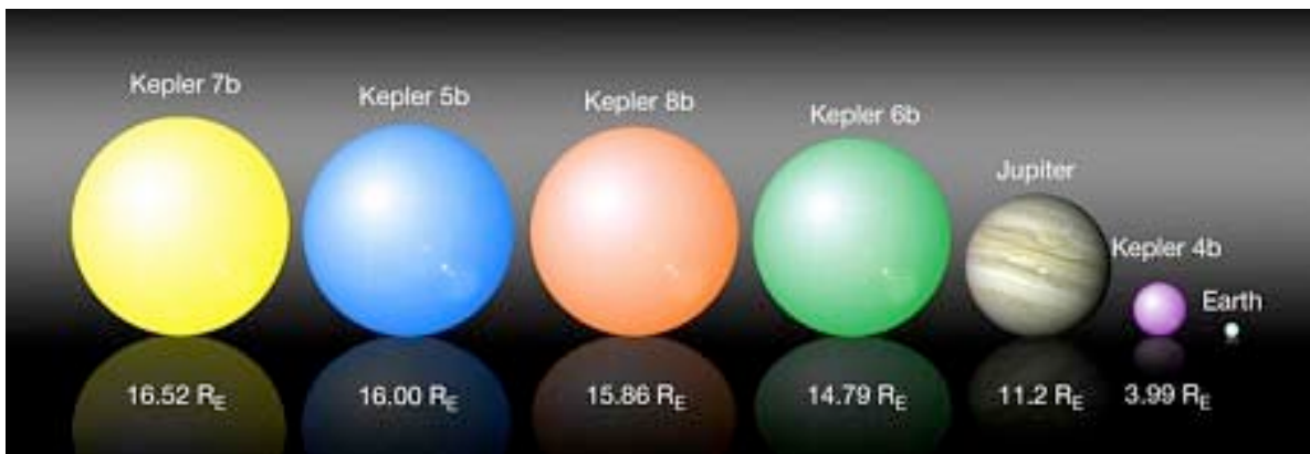
Five new exoplanets. The Kepler Mission announced the discovery of these planets, compared here with Jupiter and Earth, in early 2010. Credit: NASA Kepler Mission.
